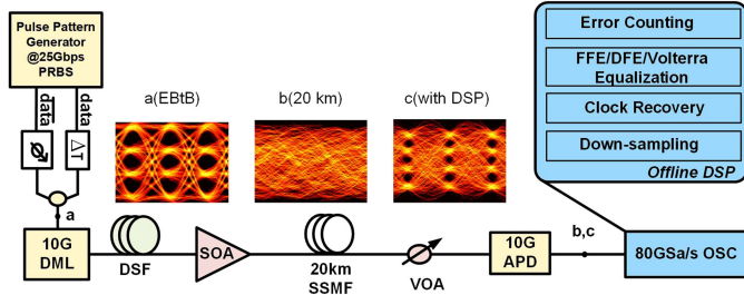
Fig. 4. Experimental setup. (a) Electrical eye diagram at the input of the DML and eye diagrams after 20km. SMF transmission. (b) Without DSP. (c) With DSP.
